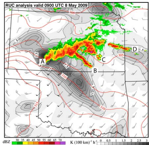
Figure 9. RUC analysis of 2D frontogenesis shaded and contoured every 0.25 \text{ K (100km)}^{-1} \text{ h}^{-1} , wind vectors (full barb = 5 \text{ m s}^{-1} , pennant = 25 \text{ m s}^{-1} ), and potential temperature (red contours every 2.5 K) on the 825-hPa surface valid 0900 UTC 8 May 2009, with NMQ composite reflectivity overlaid.
